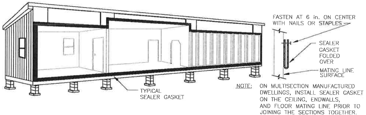
Figure 5-1.2 Typical Marriage Line Seal
