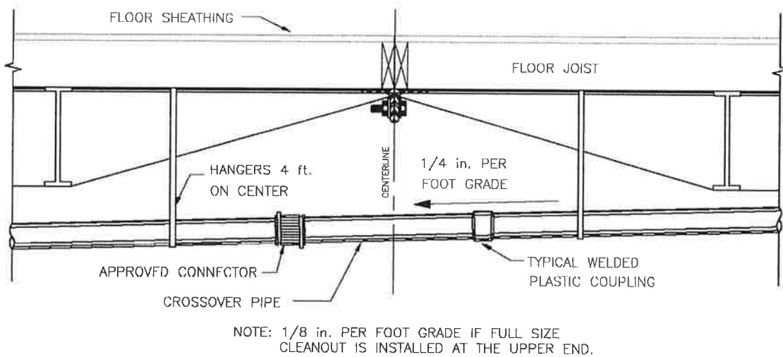
Figure 7-8.1 Typical Drain Line Support and Crossover Connection
