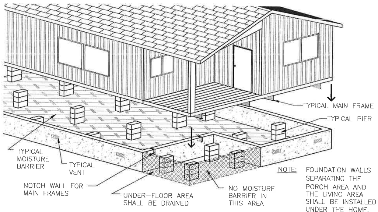
Figure 4-9.2 Under-Floor Separations
