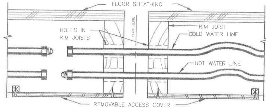
Figure 7-4.1 Typical Water Line Crossover Connection
