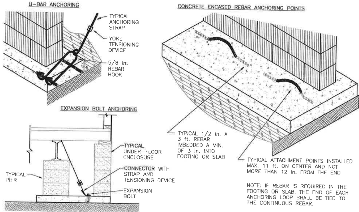
Figure 3-2.6 Typical Foundation Anchoring
