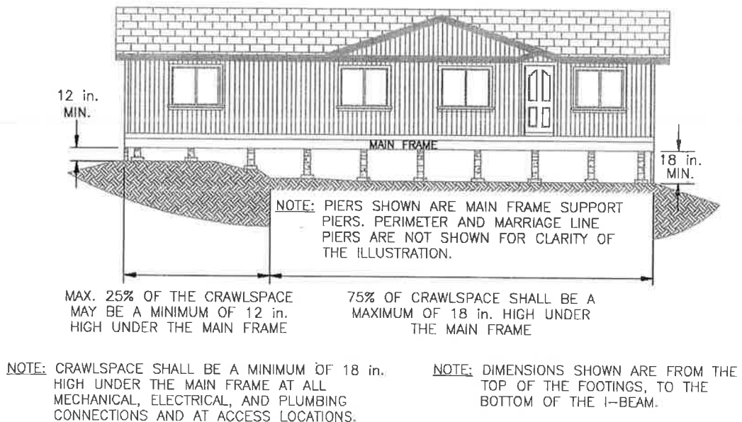
Figure 3-5.1 Minimum Under-Floor Clearance
