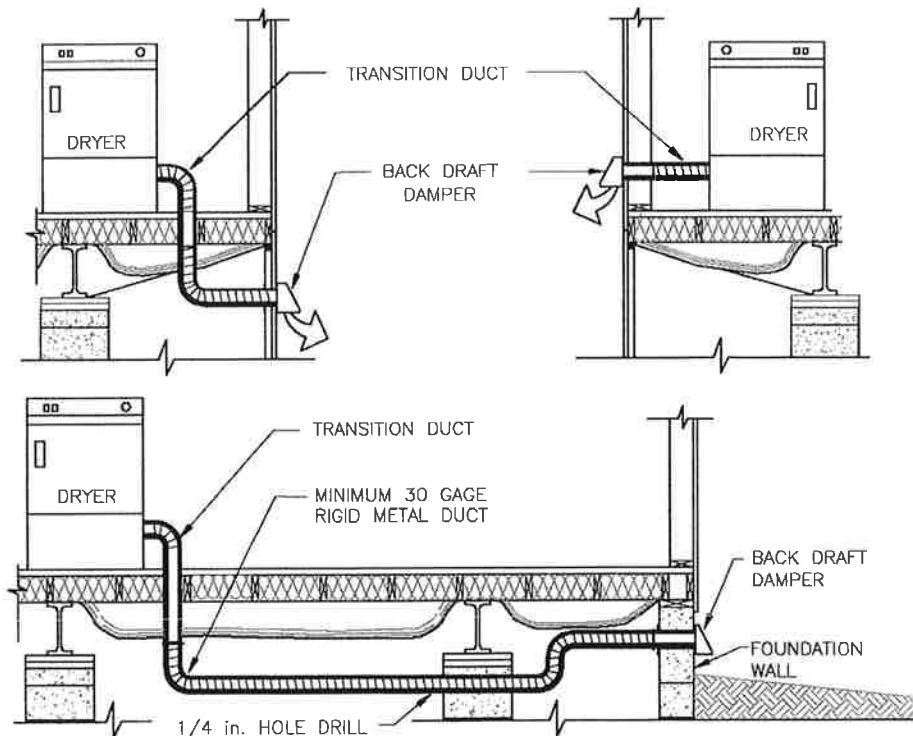
Figure 9-1.1 Typical Dryer Exhaust Duct Installation
