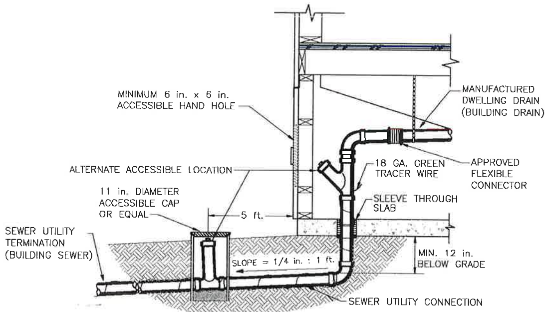
Figure 7-6.2 Typical Drain Line Connection
