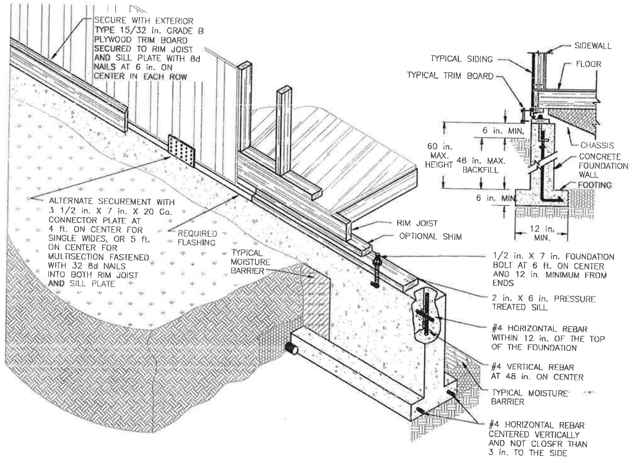
Figure 4-3.2(a) Concrete Foundation Wall Detail
