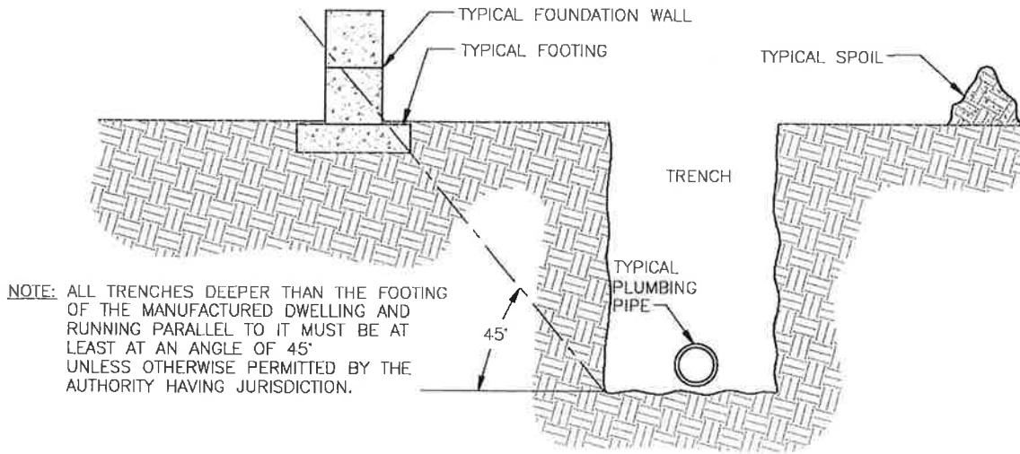
Figure 7-7.1 Typical Footing Setback from Trench
