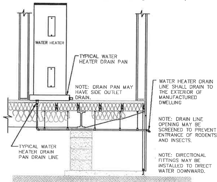
Figure 9-6.3 Typical Water Heater Drain Pan Drain Line
