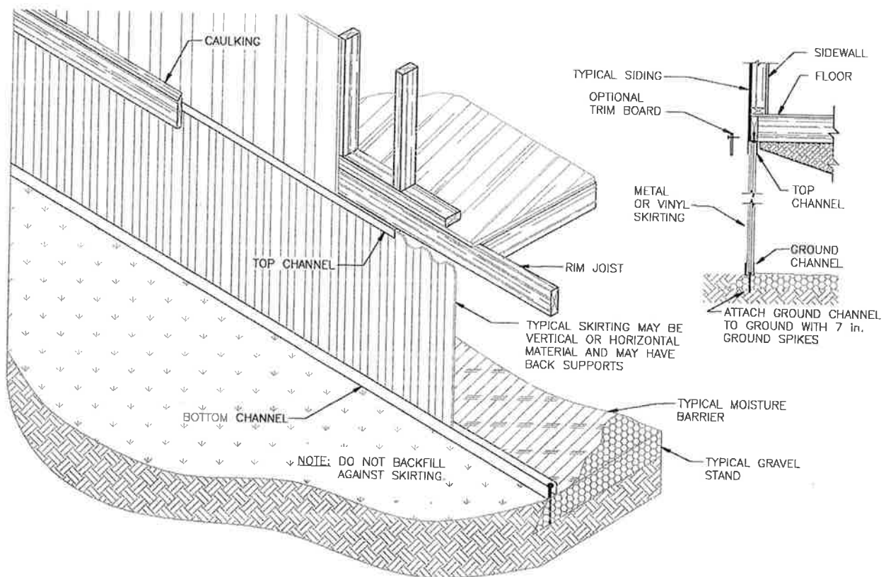
Figure 4-5.2 Typical Non-Structural Metal or Vinyl Skirting Detail
