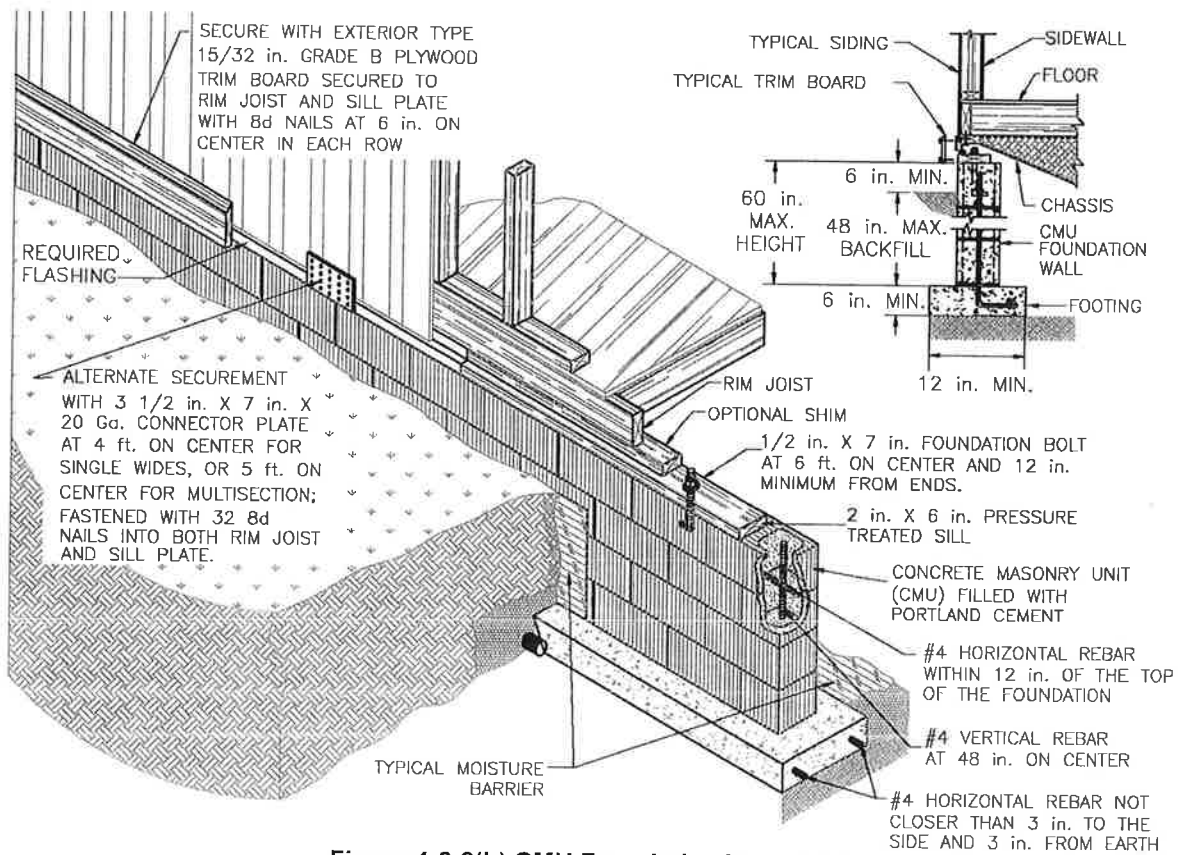
Figure 4-3.2(b) CMU Foundation Wall Detail
