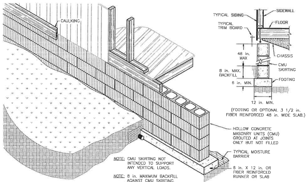
Figure 4-7.1 Concrete Masonry Block (CMU) Skirting Detail
