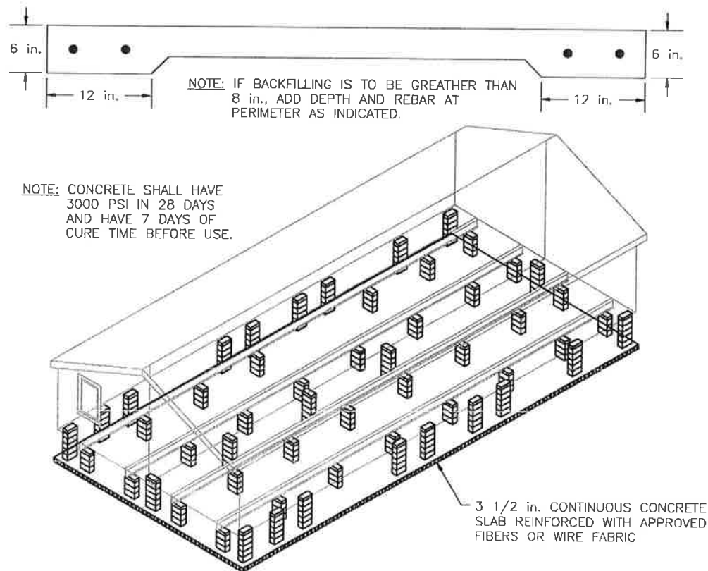
Figure 3-6.2(d) Typical Fiber Reinforced Concrete Slab Footing
