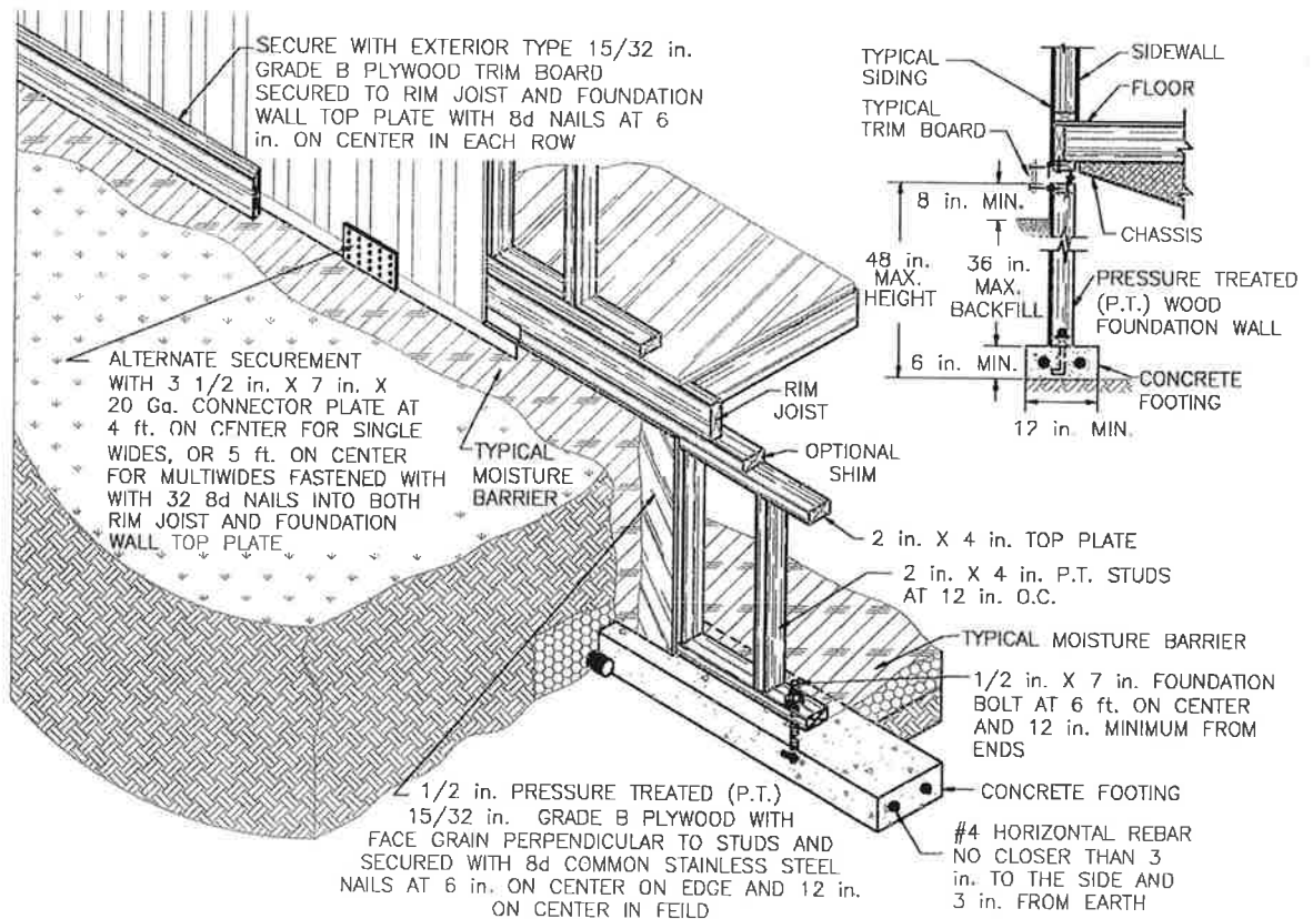
Figure 4-3.2(c) Pressure Treated Lumber Foundation Wall Detail
