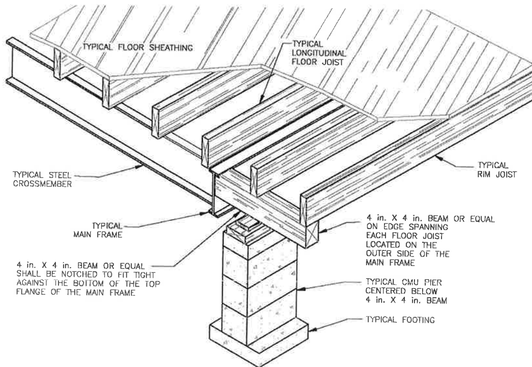
Figure 3-9.2(b) Typical Recessed Pier Detail for Longitudinal Floors
