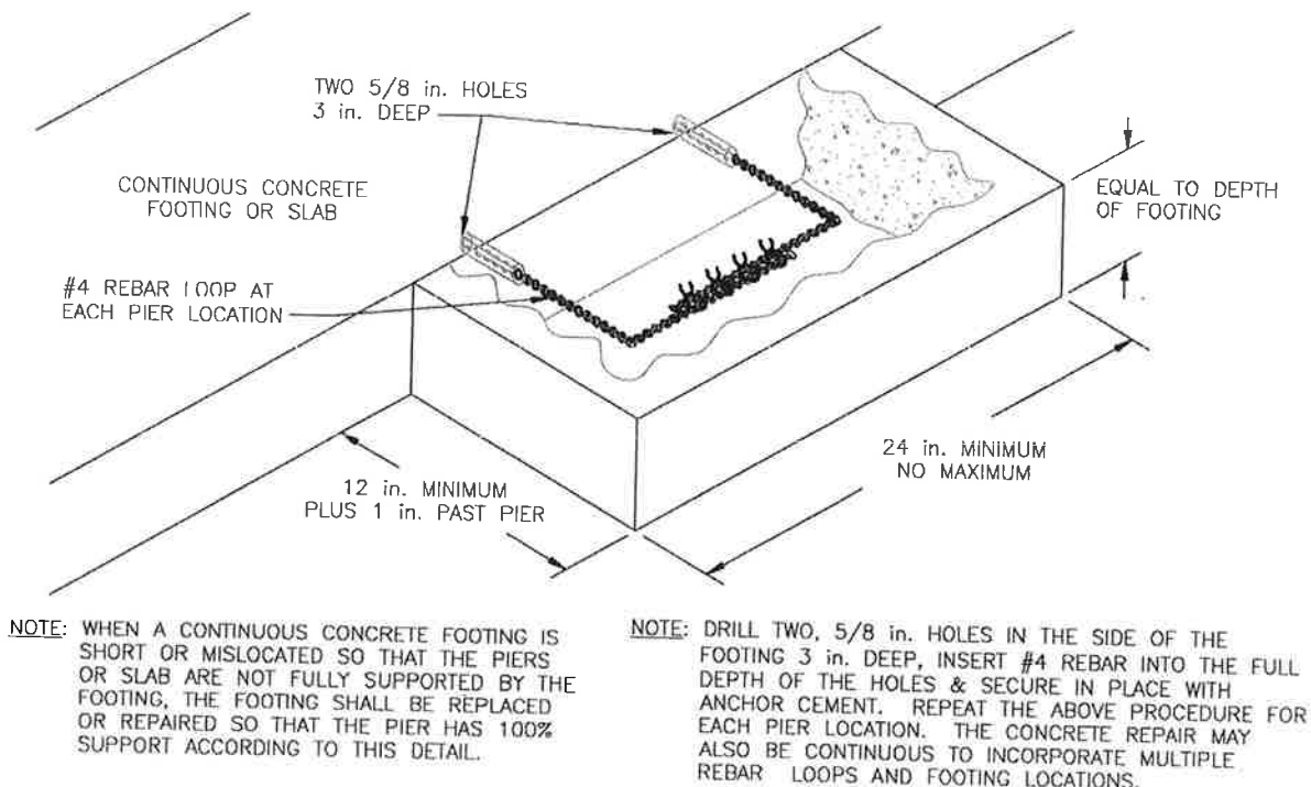
Figure 3-6.1 Continuous Concrete Footing or Slab Repair Detail
