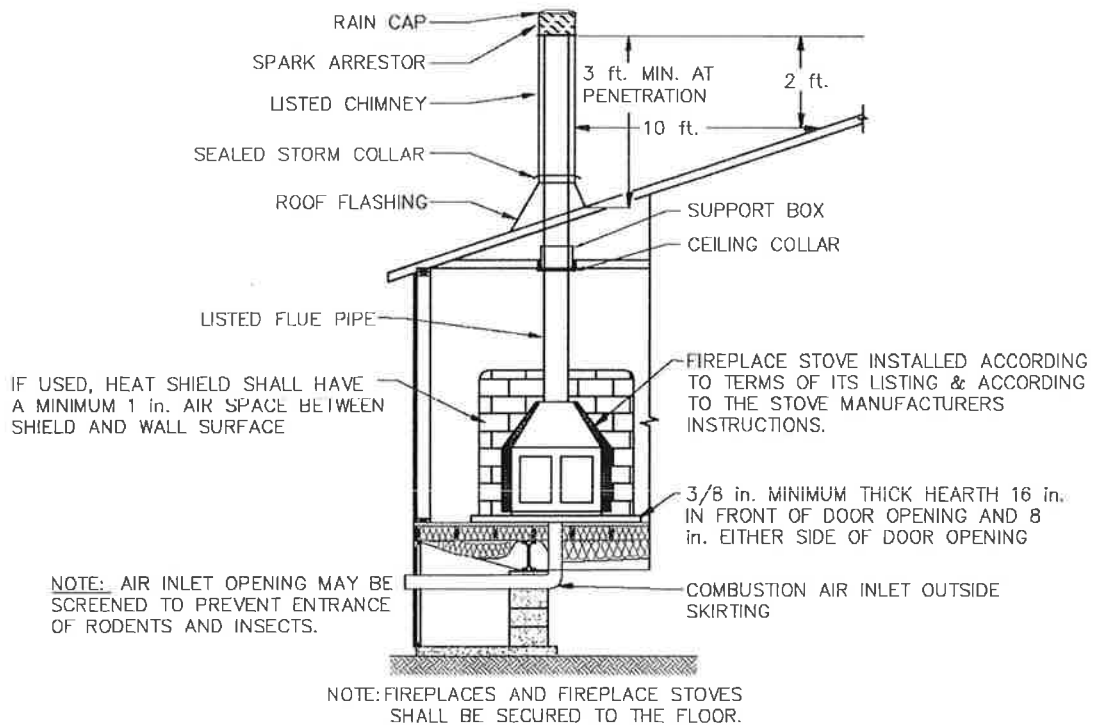
Figure 9-3.3 Typical Fireplace Stove Installation
