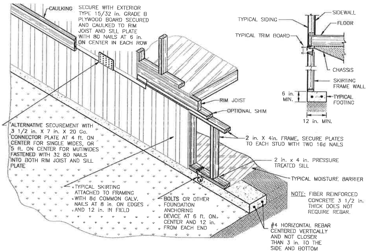
Figure 4-4.2 Structural Skirting Detail
