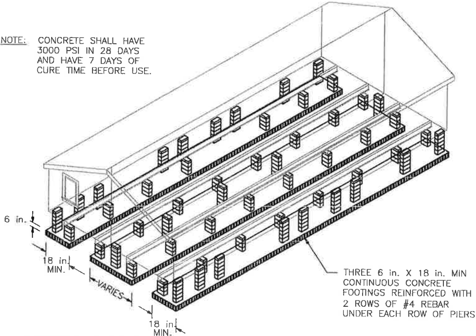
Figure 3-6.2(b) Typical Combined Continuous Concrete Footings (Three-Pad-Pour)
