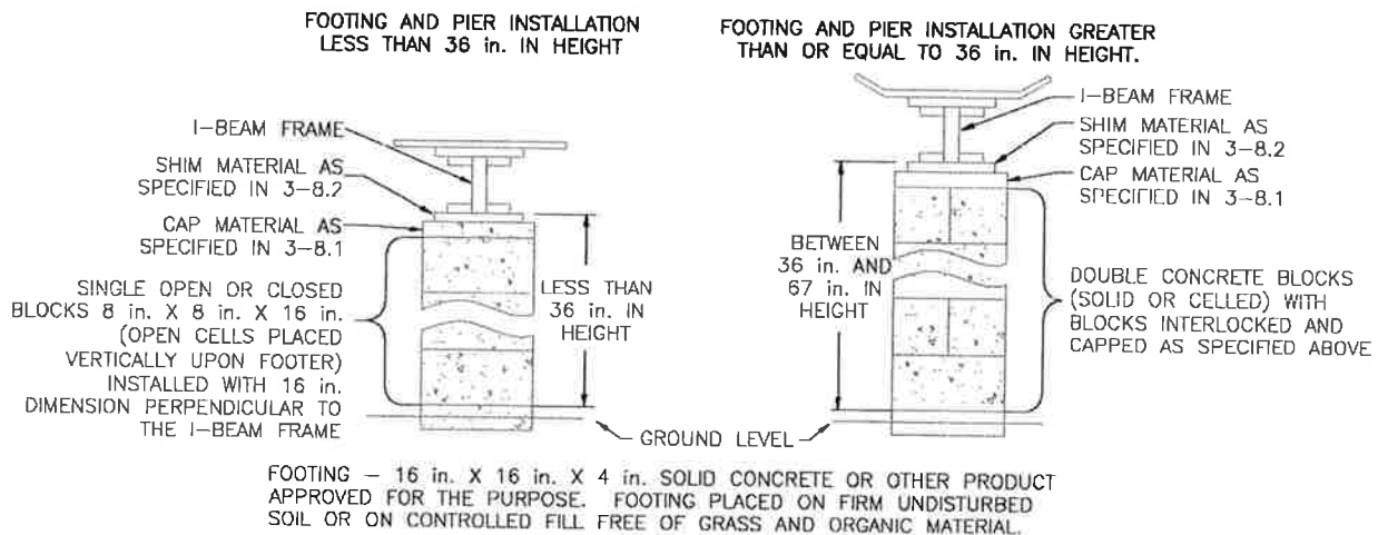
Figure 3-7.2 Typical Footing and Pier Installation
