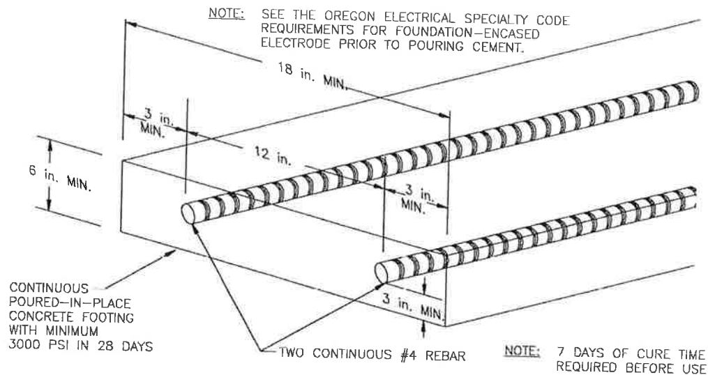
Figure 3-6.2(a) Typical Individual Continuous Concrete Footing
